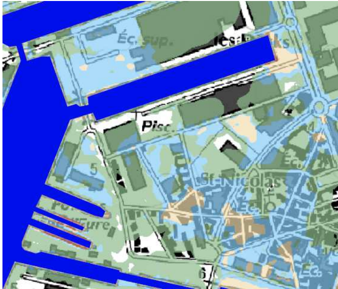
Aléa submersion marine 2100
